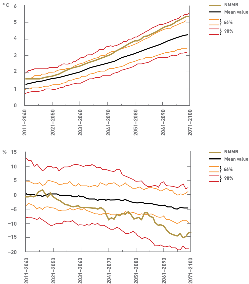
FIGURE 5.21 Extent of possible change in mean annual temperatures and precipitation for the period 2011–2100 compared to the period 1971–2000, according to scenario RCP8.5, based on the results of the 18 different models that were part of the EURO-CORDEX project
