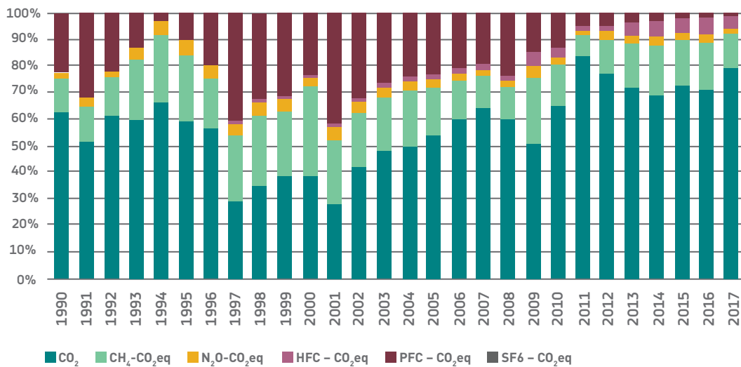
FIGURE 3.5 Share of GHG emissions within total CO 2 eq emissions, 1990–2017
